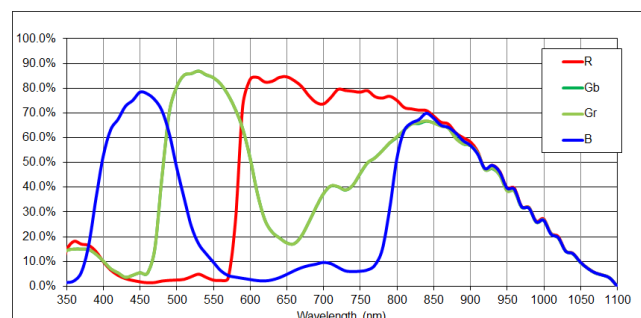
MV-CS050-60GC
